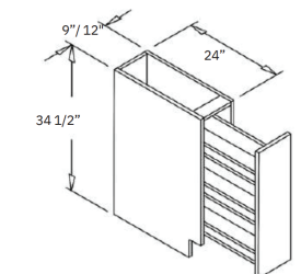
Pantry Pullout Base 34 1/2"H x 24"D
