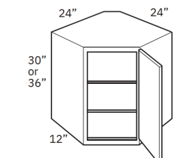
Diagonal Wall 1 Door 30", 36"H x 12"D
