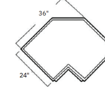
Lazy Susan 2 Doors Base 34 1/2"H x 24"D
